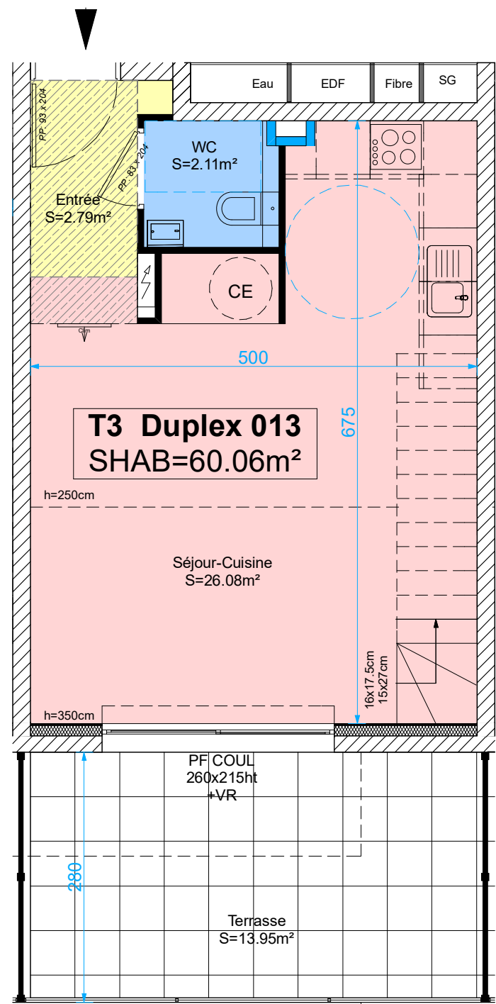
Plan R+1
